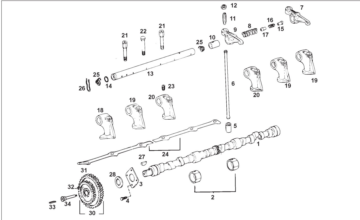
ENGINE TIMING (CAMSHAFT & COMPONENTS)
