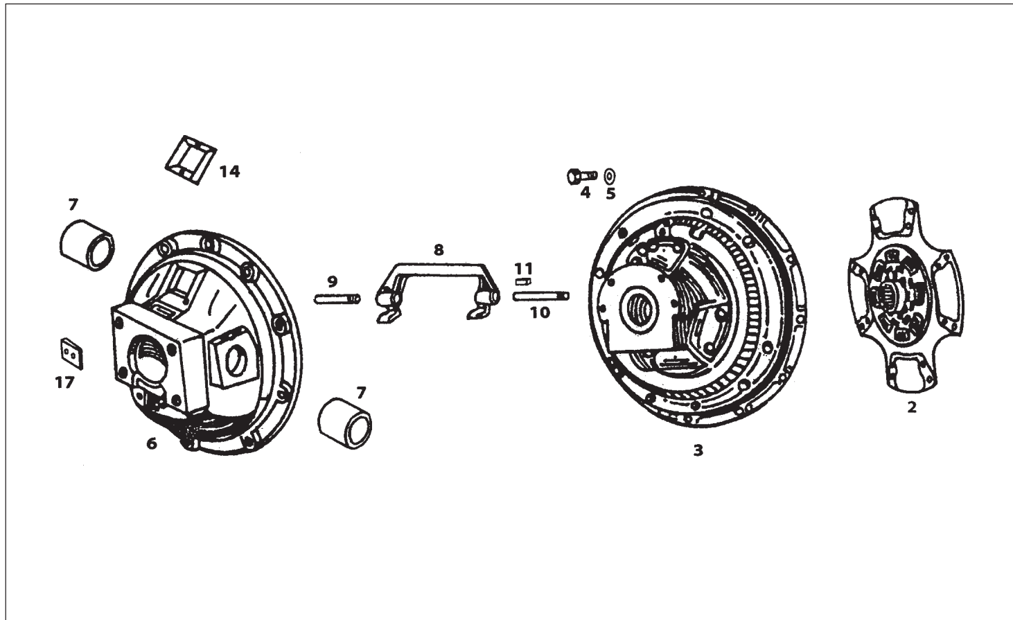
CLUTCH (352 DIA) COIL TYPE
